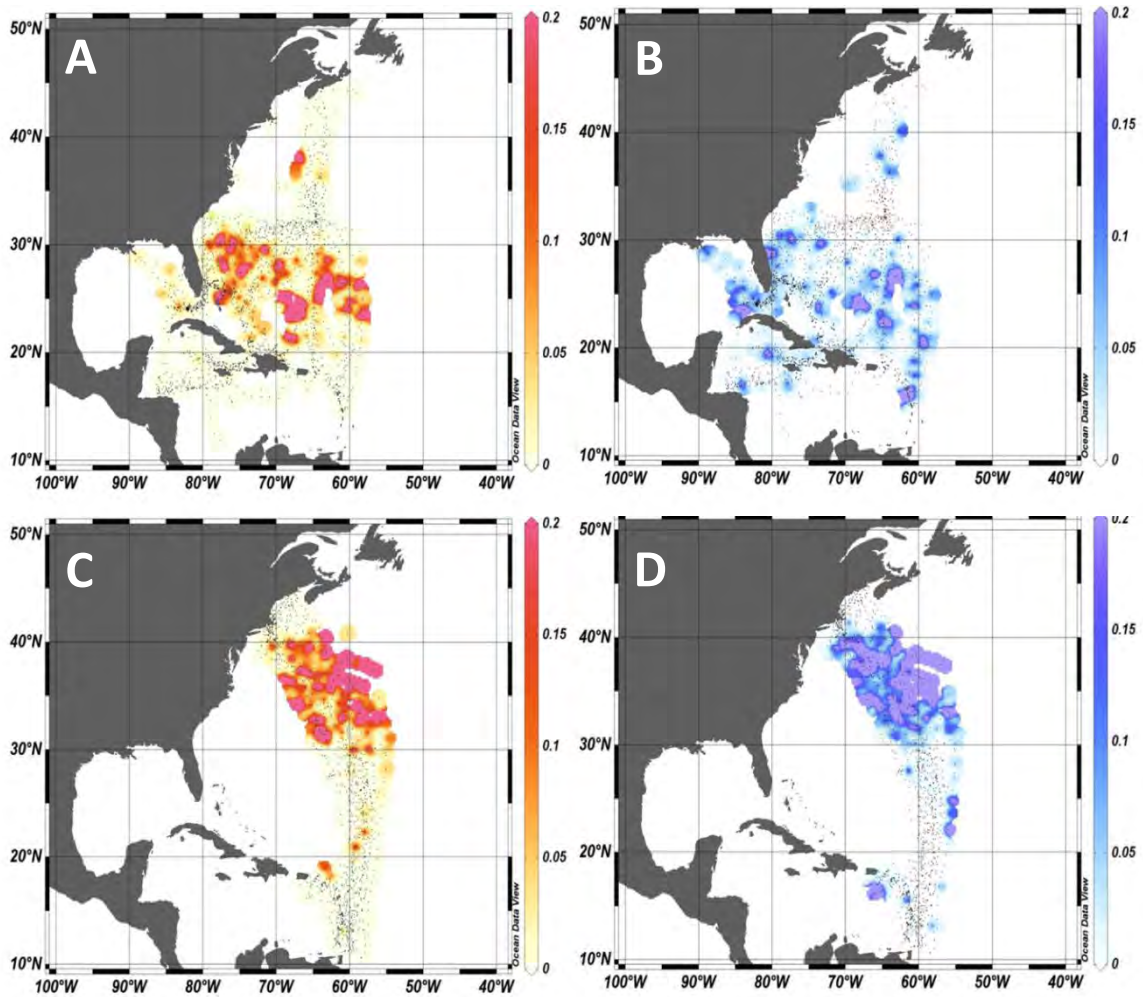
Figure 3: Distribution of Sargassum in the Sargasso Sea ( \text{g}/\text{m}^2 ) (1992-2013) shows seasonal shift. (A) S. natans , spring, (B) S. fluitans , April – early June, (C) S. natans , late October – early November, (D) S. fluitans , fall (Goodwin, Schell, & Siuda 2014, with permission). Forms were not specifically identified during this collection period.
