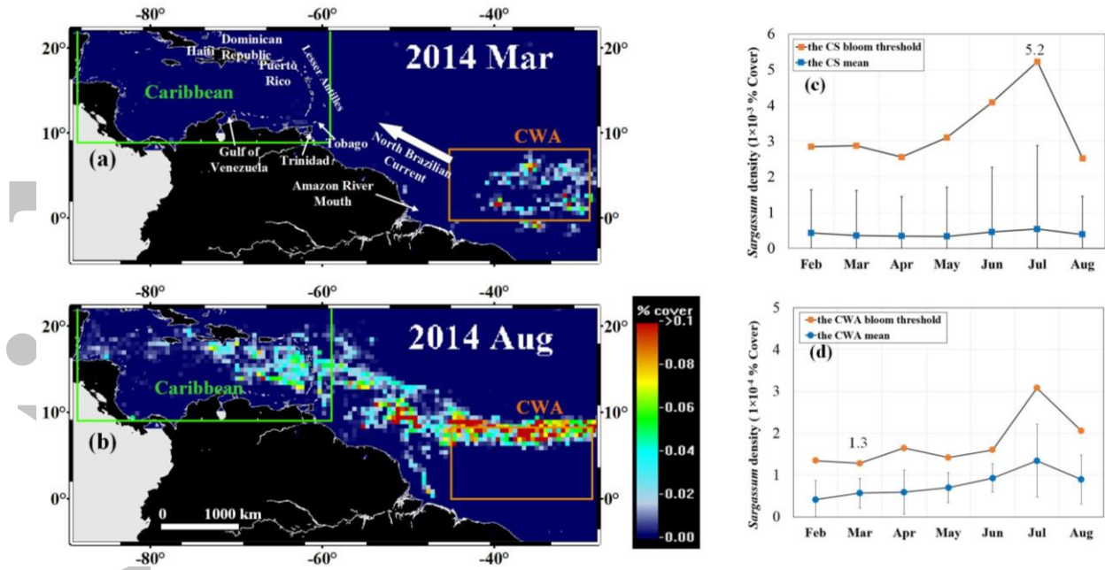
Figure 1. Sargassum area density (% cover) maps in March 2014 (a) and August 2014 (b) derived from MODIS observations [Wang and Hu, 2016], suggesting Sargassum transport from the CWA to the CS following dominant winds and currents (white arrow). The green box and orange box delineate the CS and CWA hotspot regions, respectively. (c) and (d) are Sargassum density thresholds used to determine blooms and non-blooms in the 1^{\circ} \times 1^{\circ} grids of the CS and in the CWA hotspot region, respectively. Vertical bars represent standard deviations of each month of 2000 - 2010 (non-bloom years). The bloom threshold was determined as the mean plus 2 standard deviations. For example, in July, if the density in any grid in the CS is > 5.2 \times 10^{-3} \% , it is considered as a bloom in that grid; in March, if Sargassum density in the CWA hotspot is > 1.3 \times 10^{-4} \% , it is considered as a bloom.
