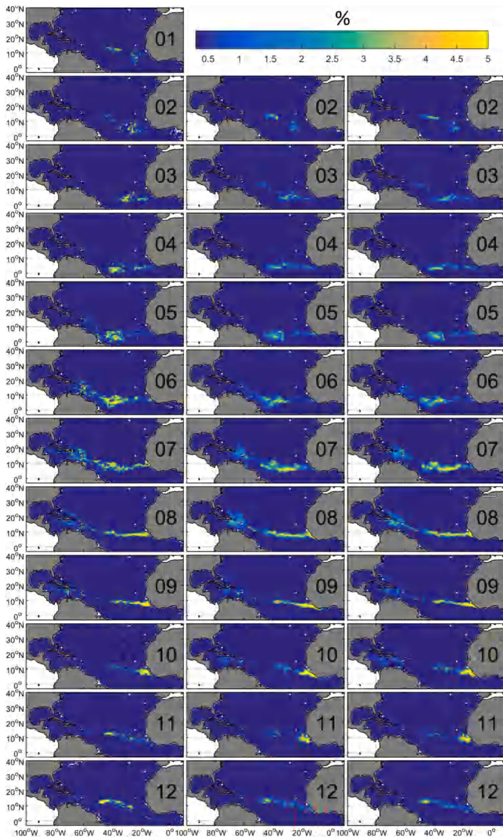
Fig. 3. Observed and simulated Sargassum monthly distribution in 2017 expressed as the proportion of pixels containing Sargassum . Simulations show Sargassum distribution forecast from observations made in the previous month (Exp1). Satellite monthly composite (left column), simulated monthly composite (middle) and simulated monthly composite including 1% windage (right column). The initial positions for Lagrangian simulations are taken from the satellite monthly composite for each month from January to November 2017.
