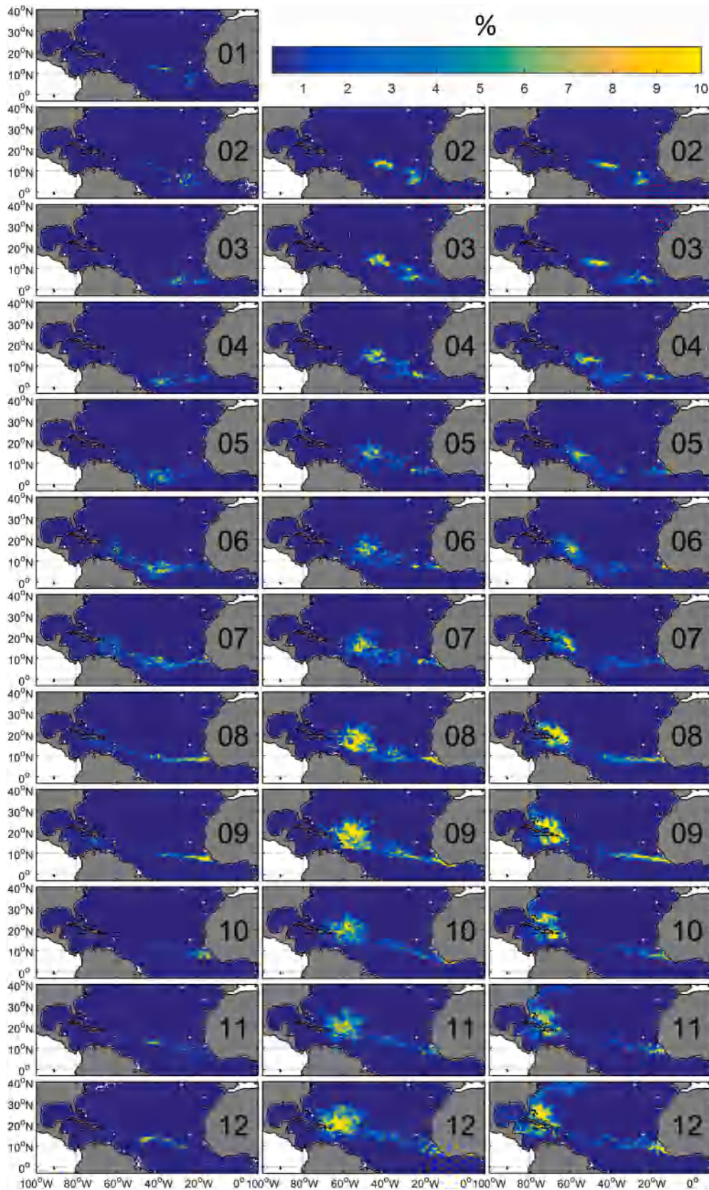
Fig. 4. Observed and simulated Sargassum monthly distribution in 2017 expressed as the proportion of pixels containing Sargassum . Simulations show Sargassum distribution forecast from observations made in January (Exp2). Satellite monthly composite (left column), simulated monthly composite (middle) and simulated monthly composite including 1% windage (right column).
