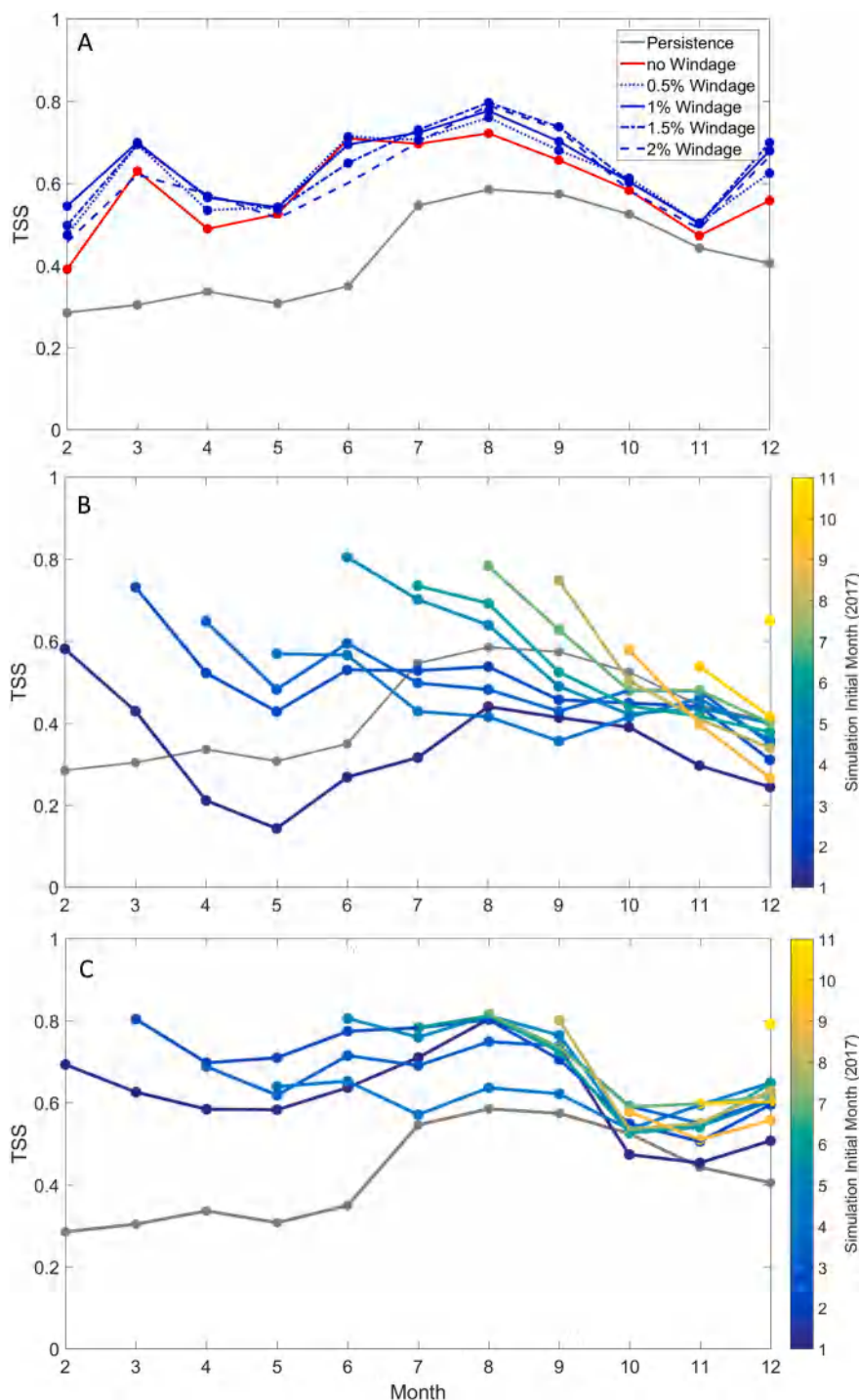
Fig. 2. Skill diagnostic of simulations. A) Exp1. Comparison between simulated monthly composite and satellite monthly composite at month j + 1 for different windage values, from February to December 2017. The TSS for persistence is in grey. B) and C) Exp2. Comparison between simulated monthly composite and satellite monthly composite, for long simulations, initialized from February to December 2017. No windage (B) and 1% windage (C). The TSS for persistence is in grey.
