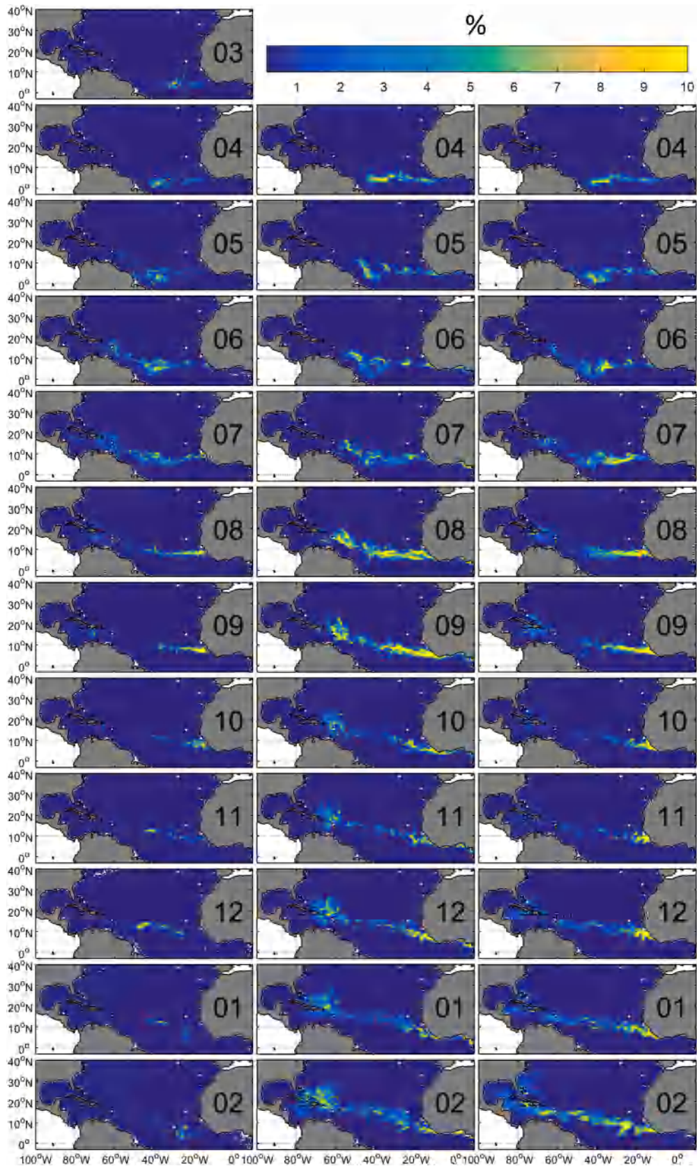
Fig. 5. Same as Fig. 4. with simulations starting from observations made in March (Exp2). Note that for the period after December 2017, year 2017 is repeated for currents and satellite monthly composites.
