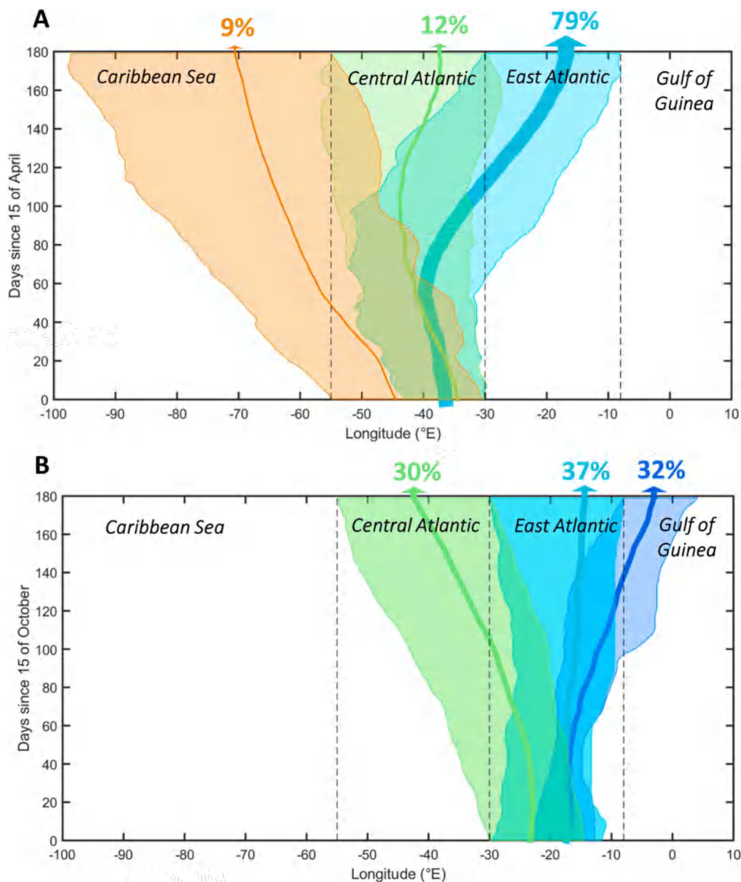
Fig. 7. Main pathways of Sargassum to the 4 zonal regions (see text) and fluxes over 6 months drift from Exp2. The envelope of Sargassum trajectories is shown, with the thickness of the central line following the percentage of Sargassum reaching the region after 6 months. A) Pathways of Central Atlantic Sargassum in April, B) Same as A) for Sargassum present in the East Atlantic in October.
