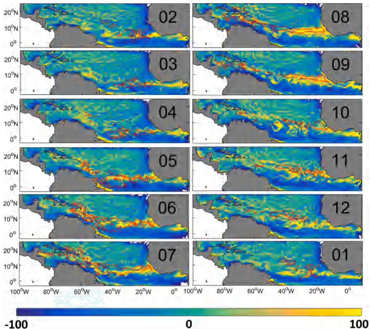
Fig. 8. Sargassum monthly distribution in 2017, starting from homogeneous initial positions (Exp3). The background color is the ratio between final and initial density, in %. The red contour lines overlaid correspond to the area of Sargassum presence from satellite monthly composite. (For interpretation of the references to color in this figure legend, the reader is referred to the web version of this article.)
