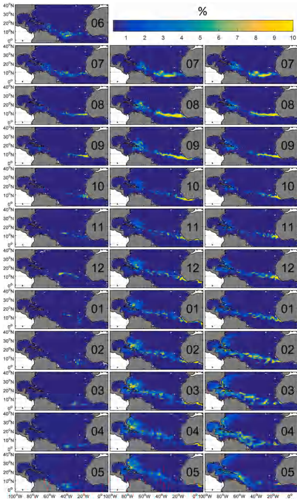
Fig. 6. Same as Fig. 4. with simulations starting from observations made in June (Exp2). Note that for the period after December 2017, year 2017 is repeated for currents and satellite monthly composites.
