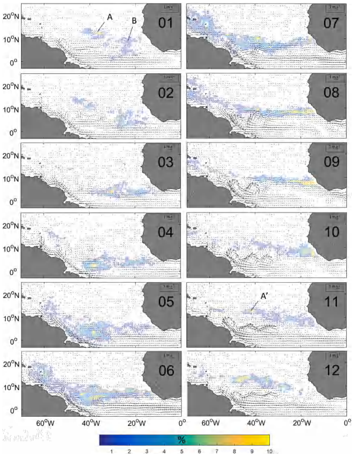
Fig. 1. Sargassum monthly distribution in 2017 expressed as the proportion of pixels containing Sargassum . Satellite monthly composite with monthly average model surface currents overlaid as black vectors.
